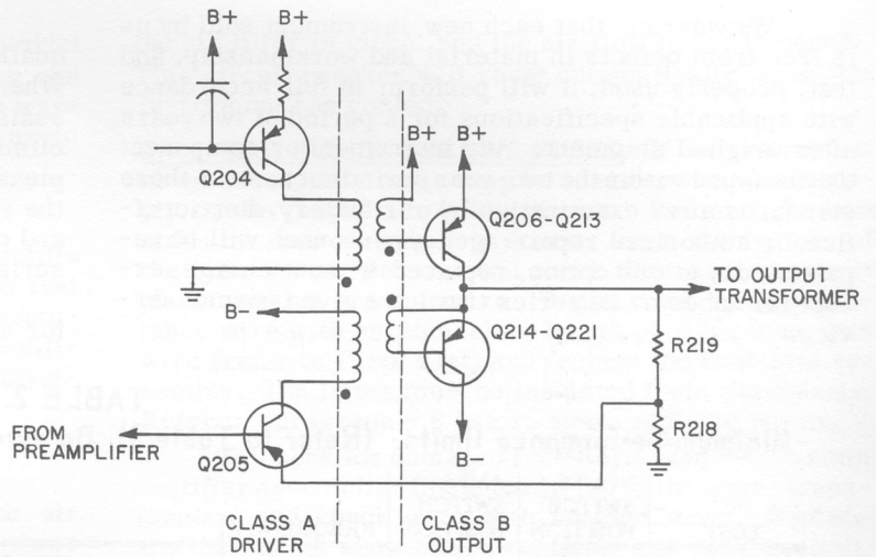
Figure 4-5. Power-amplifier circuit.
