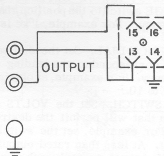
Figure 2-2. Output connections.
